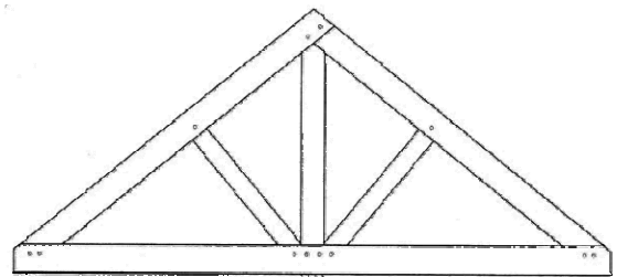
KING POST TRUSS
