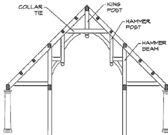
HAMMER BEAM BENT
