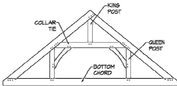
QUEEN POST TRUSS
